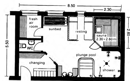
⑧ Hotel sauna 5.50 x 8.50 m
